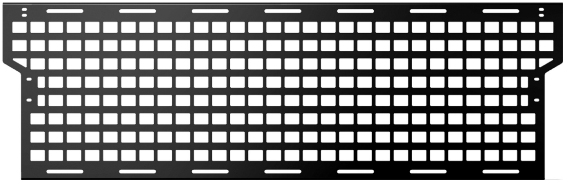
FRONT PANEL
